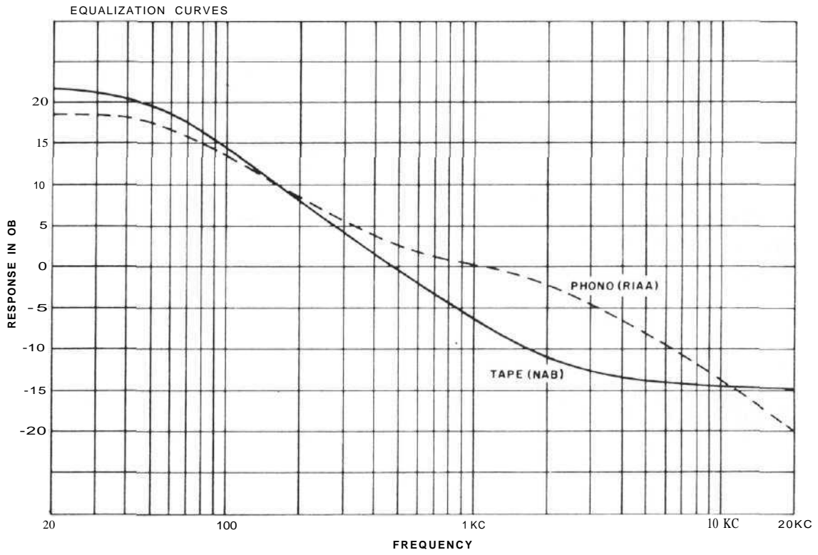
Figure 22. Equalization Curves.
