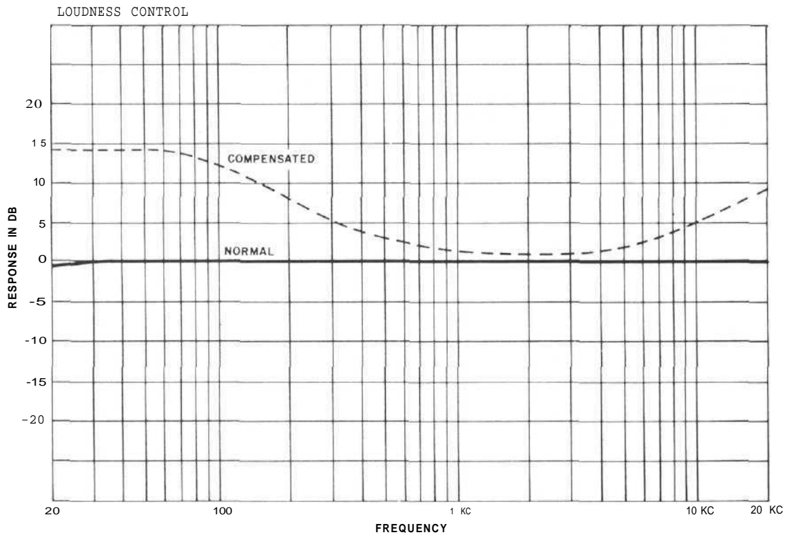
Figure 25 Loudness Control.
