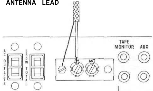
Figure 21. Connections for a 75 ohm antenna
