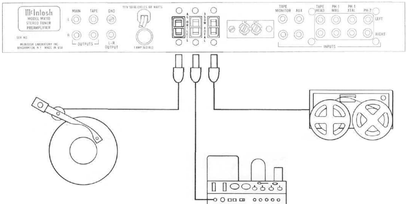
Figure 17. AC Connections.
