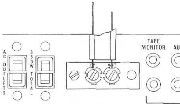
Figure 20. Connection for 300 ohm antenna
