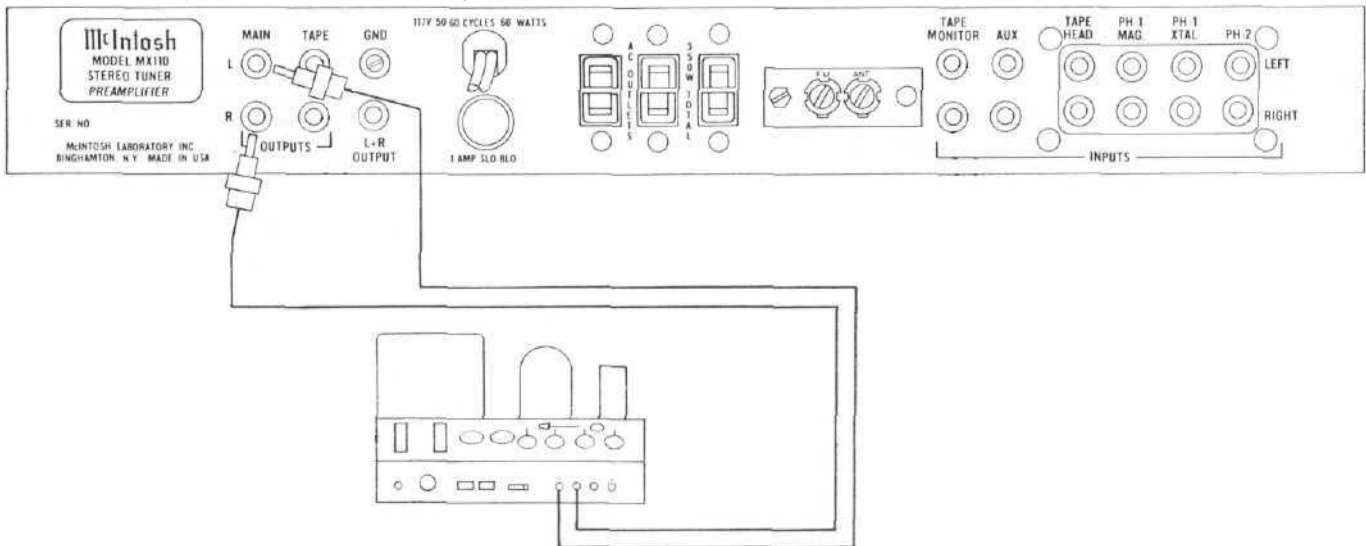
Figure 19. Output Connections
